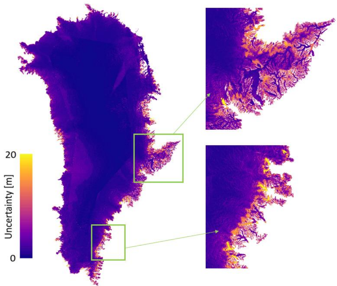
Figure 16: Uncertainty map for an example seamless product (2019), demonstrating the differing uncertainty values for CLI, EOLIS and interpolated pixels.
