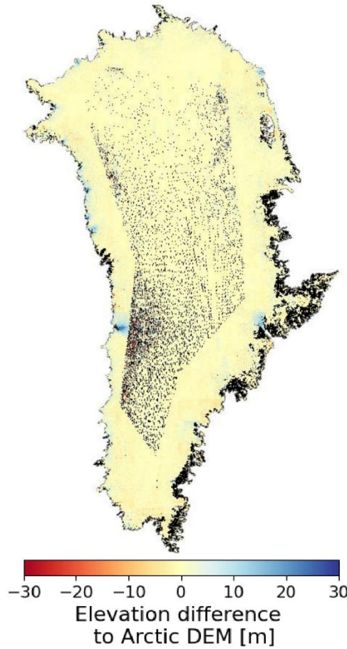
Figure 13: Elevation difference map of 2011 EOLIS annual DEM after gridding, adjusting and combining has been performed. Missing data is highlighted in black.
